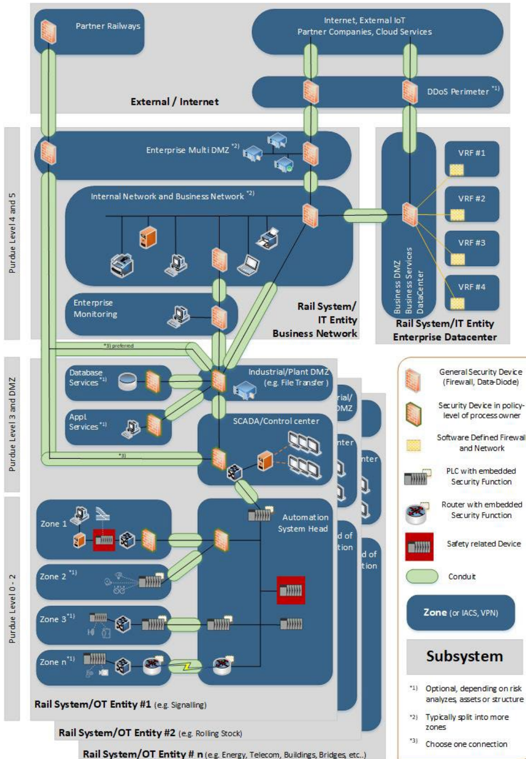
Figure 7 Example of a proposal railway system zone model concerning TS50701 (Source: CLC/TS 50701:2021 - © CENELEC, reproduced with permission)
