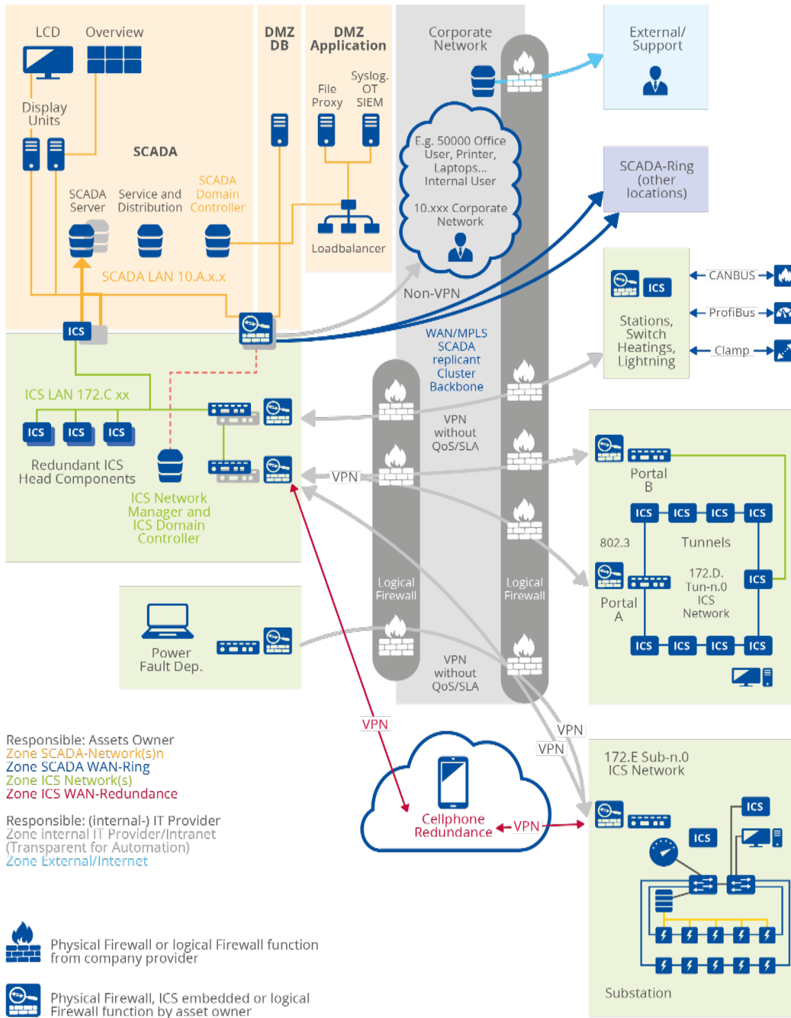
Figure 6 Simplified example of a proposal zone model for one entity
